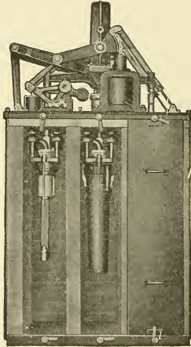
Fig. 159. 3000-Ampere, 3-Phase, Electrically-Operated Oil Circuit Breaker—1 Pole Enclosed; 1 Pole, Door Removed and Tank in Place; 1 Pole, Door and Tank Removed
